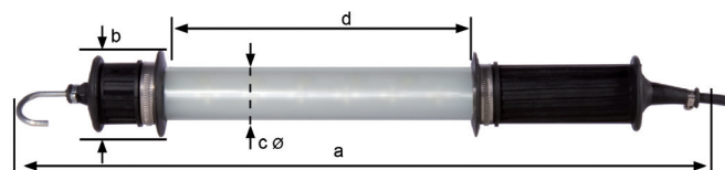
Abmessungen in mm | Dimensions in mm
