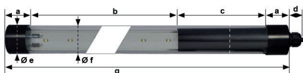
Abmessungen in mm | Dimensions in mm
